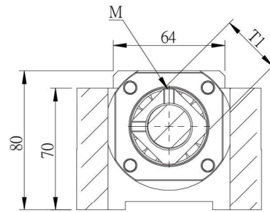
Section U-U
