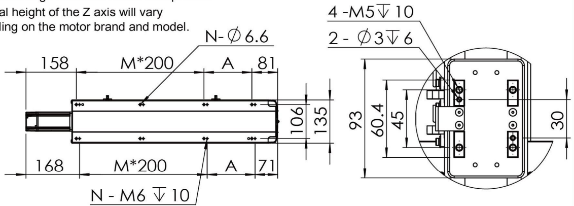
Detailed View P Scale 1 : 3
